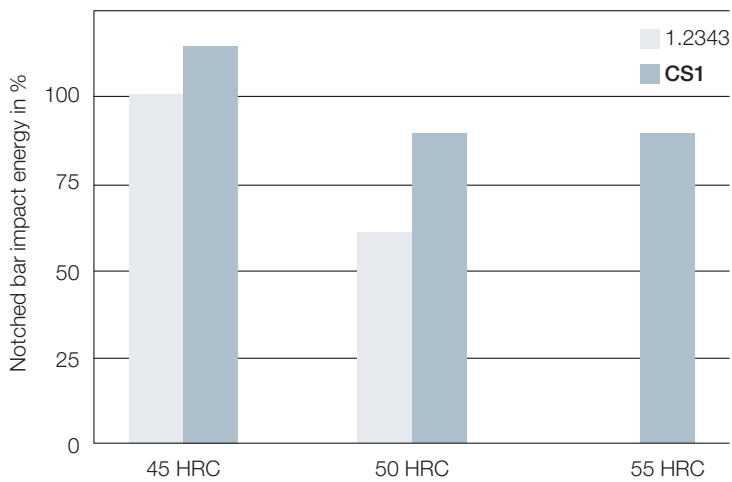
Toughness comparison
