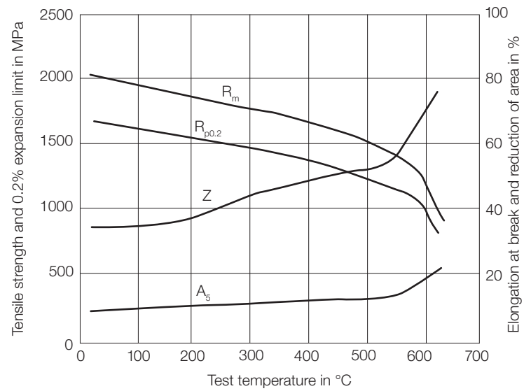
High-temperature strength diagram 56 HRC
