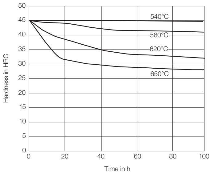
Long-term temper resistance 45 HRC
