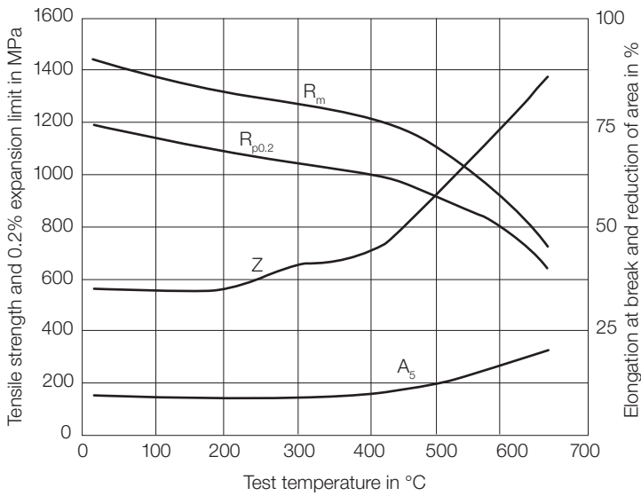
High-temperature strength diagram 45 HRC
