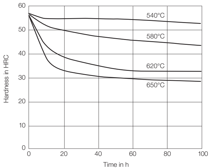
Long-term temper resistance 56 HRC
